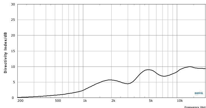
Directivity Index
